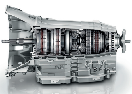
The 7G-TRONIC PLUS automatic transmission offers outstandingly smooth gear changes and tremendous potential for saving fuel. Standard on SWB and 119 LWB Van, and crewcab.
